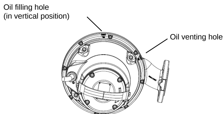
Fig. 11 Oil filling holes
